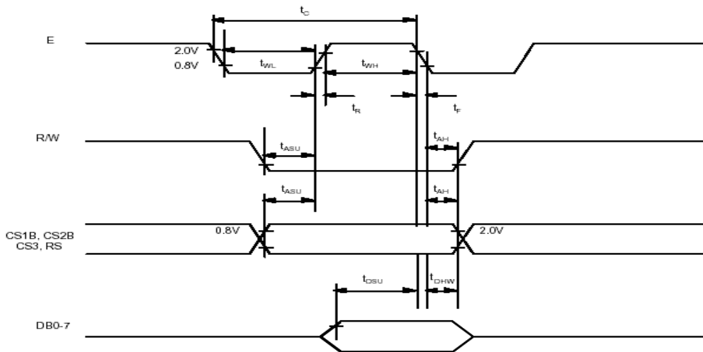
Fig 6. MPU write timing
