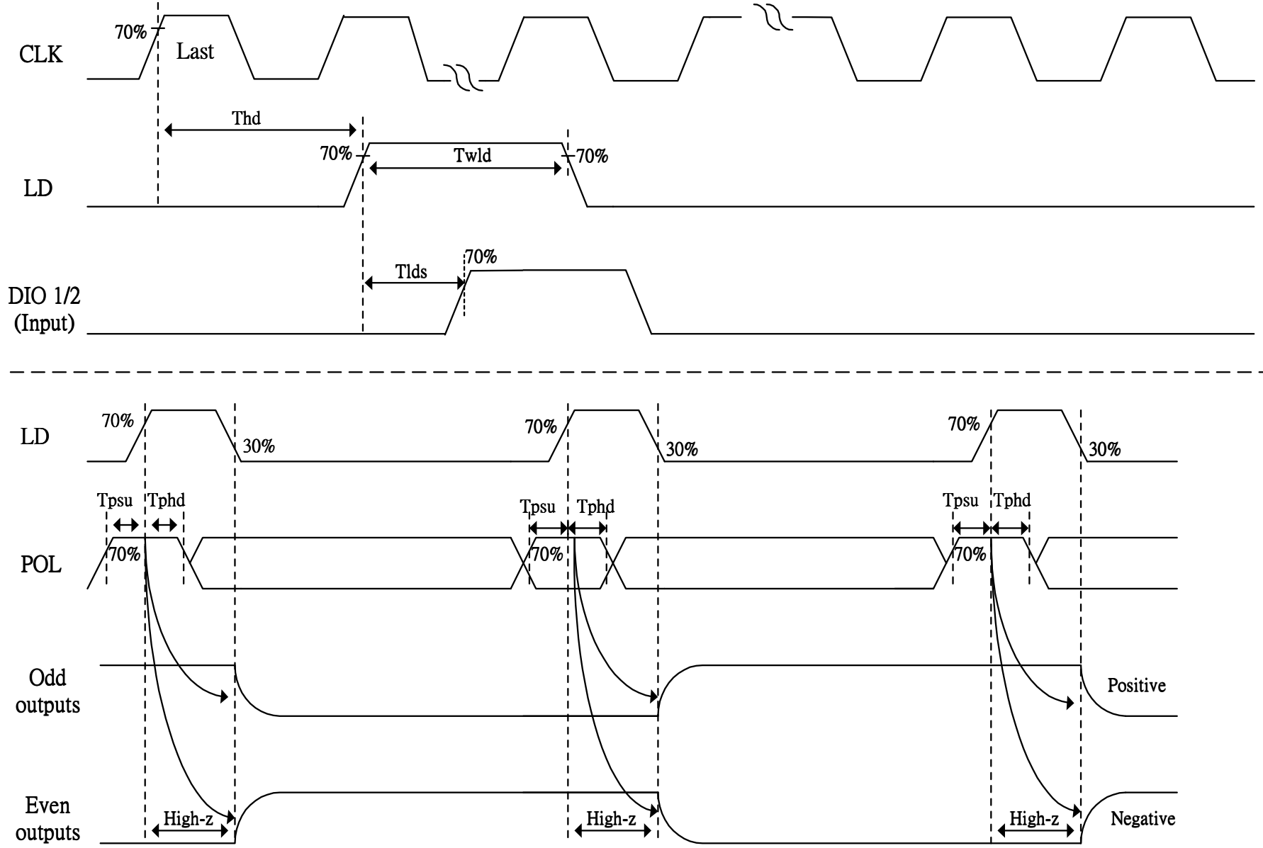
Fig. 11-2 Horizontal timing(2)
