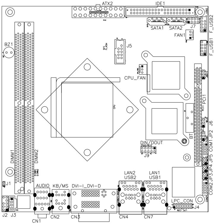
Connector Locations on MI932
