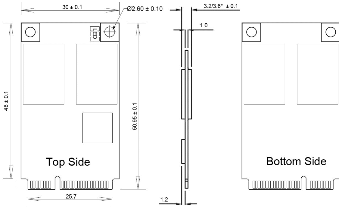
Figure 3: InnoDisk Mini PCIeDOM D150 mechanical dimensions (* thickness would be different in different capacity)
