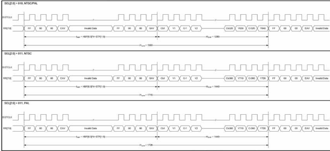
Figure 6 CCIR656 horizontal timing
