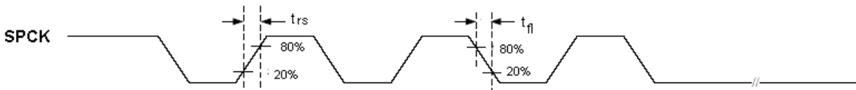
Figure 4 Rising/Falling time
