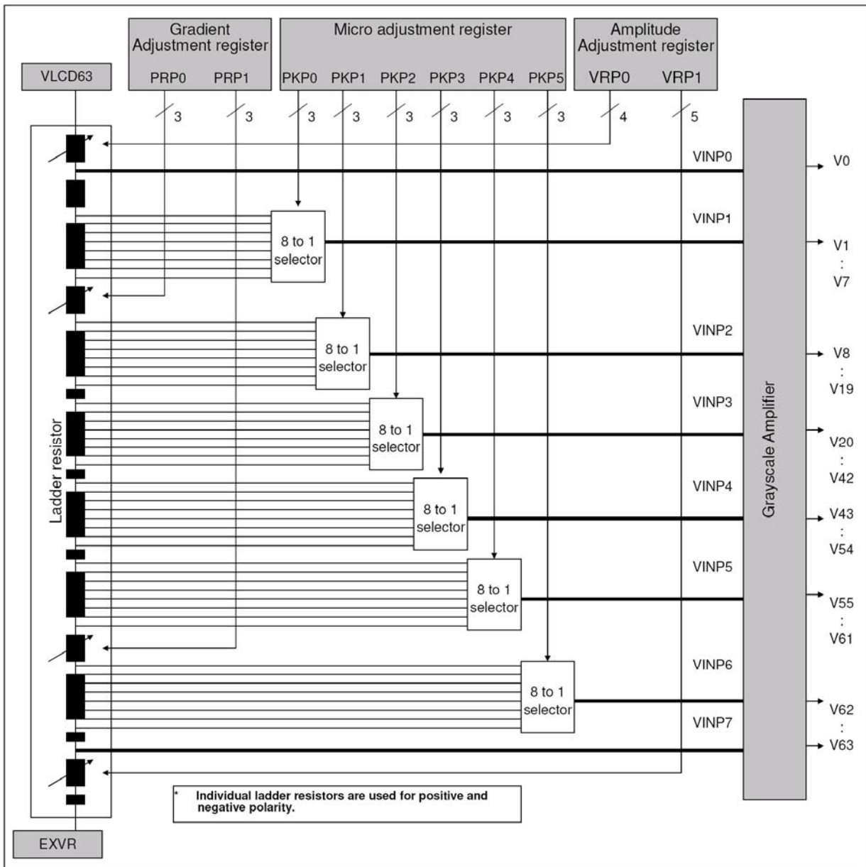
Figure 11.1-1 Grayscale amplifier
