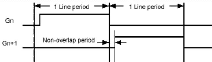
Figure 10.2-10 NO timing diagram
