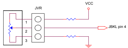
Variation Resistor
