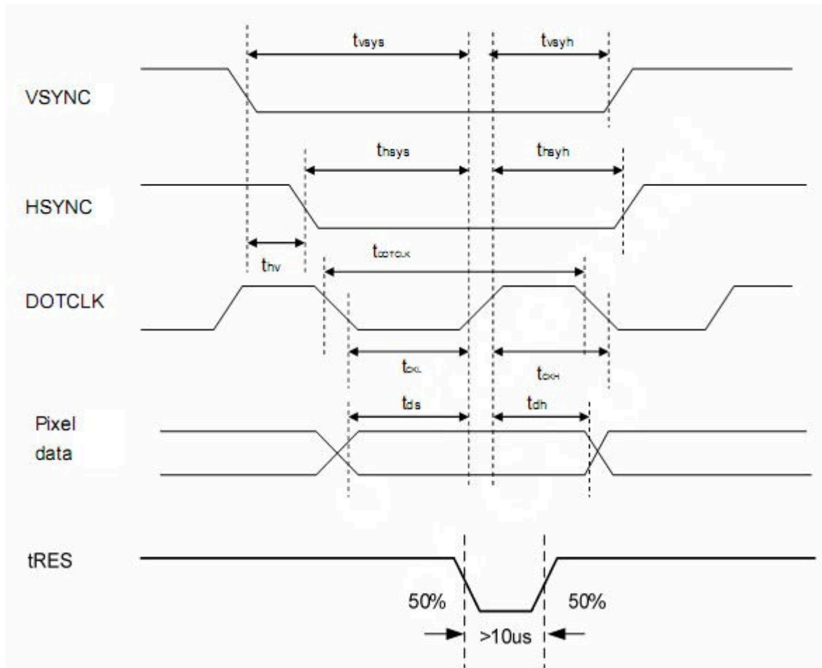
Figure 1: Pixel Timing
