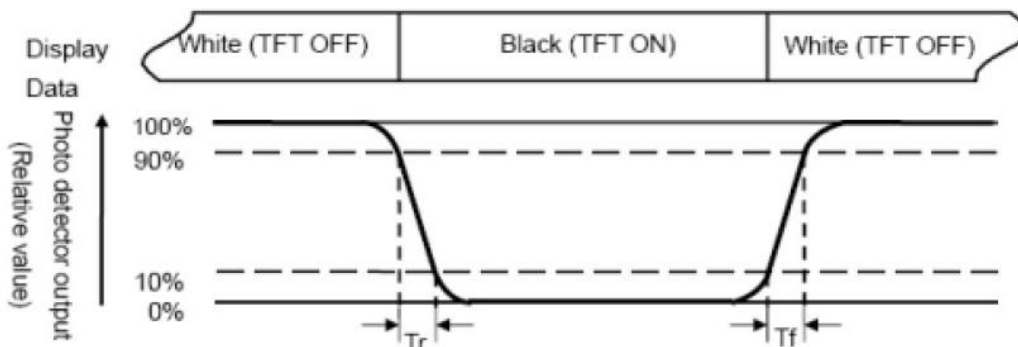
Fig 10-3 Definition of response time
