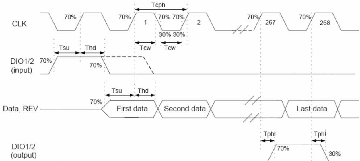
Timing diagram 1 (Default CHNSL1=H, CHNSL0=H) EDGSL= L or open
